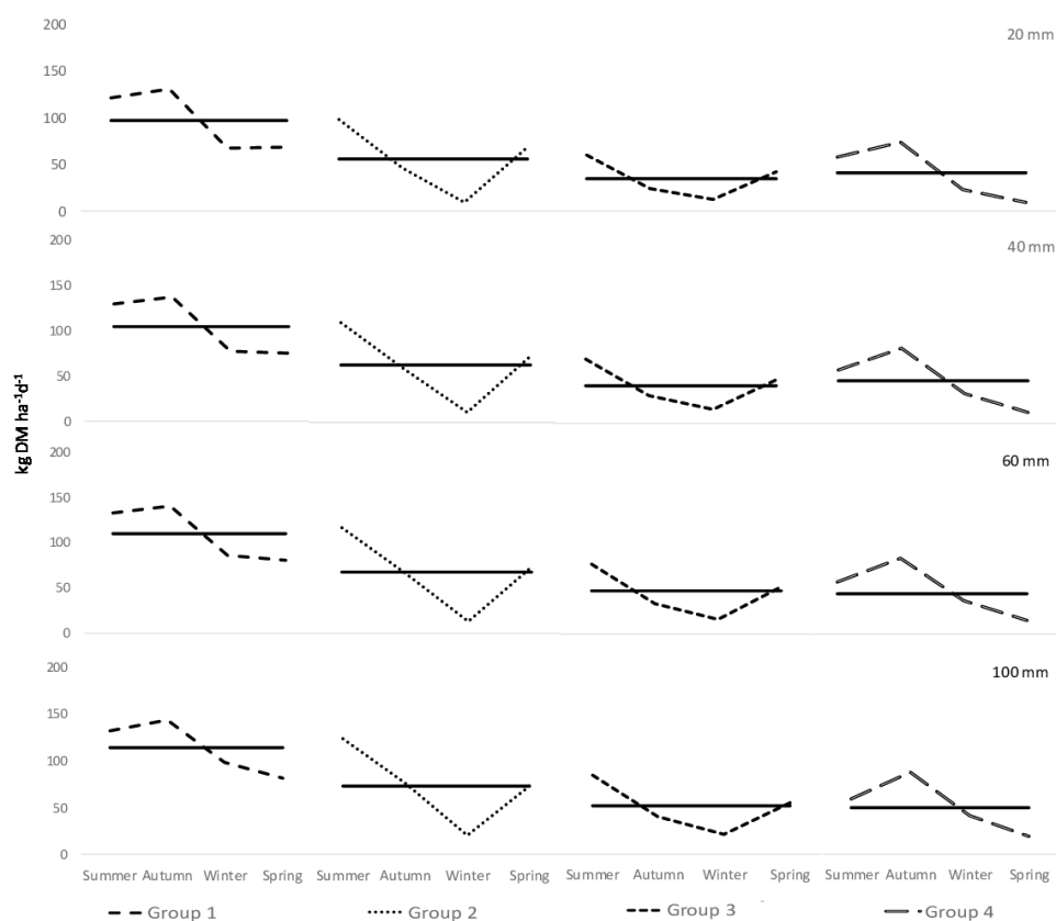
Figure 3. Herbage accumulation rate (HAR) in seasons of the year and annual mean HAR of Groups of meteorological stations in Brazil, created by cluster analysis. Dashed and solid lines correspond to season and annual mean HAR, respectively. HARs were simulated using data of 286 meteorological stations from years 1963 to 2009 by mathematical empirical model, considering four soil water holding capacities (20, 40, 60 and 100mm).
