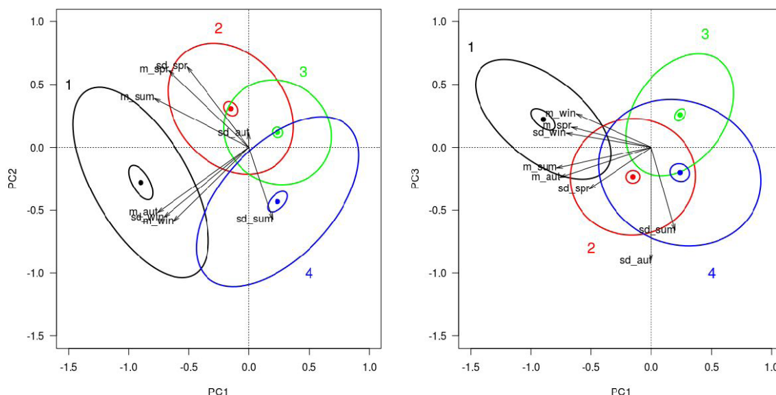
Figure 1. Biplot of the first two principal components PC1 and PC2 (a) and first and third principal components PC1 and PC3, with 95% confidence ellipses for prediction (larger diameter) and mean vector (smaller diameter) of each group considering 60mm soil holding capacity. As results for different soil water holding capacities were very similar, only results from 60 mm soil water holding capacities are presented.
