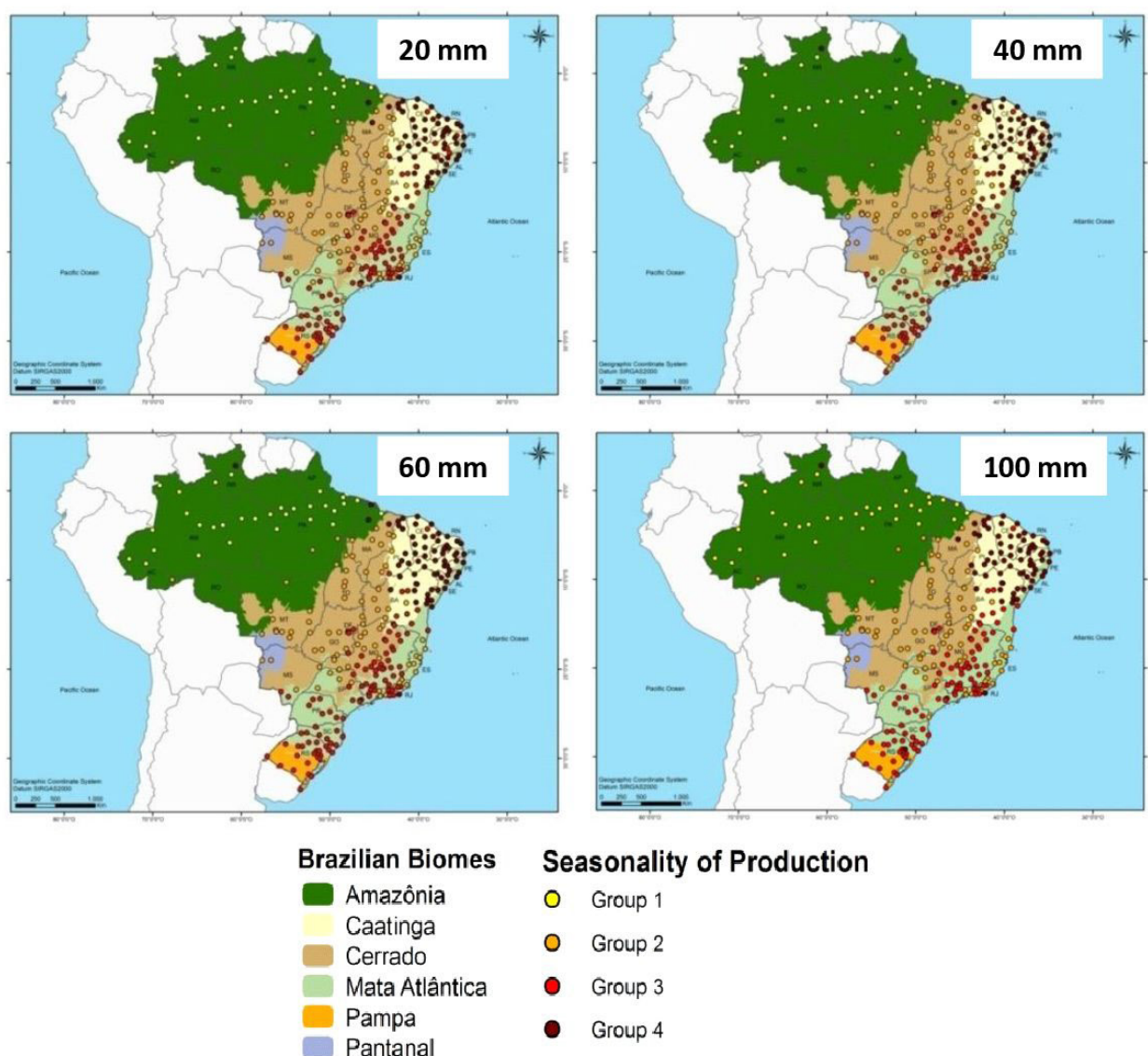
Figure 2. Classification and distribution of meteorological stations in Brazil according to cluster analysis. Cluster analysis was done according to Marandu palisade grass herbage accumulation rate mean and standard deviation in each season of the year.
